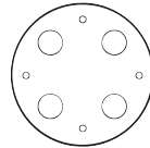
AS 24-44420 (4 x AWG 4, 4 x AWG 20)
